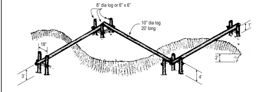
Figure E-34. Island hopper (course sketch).
